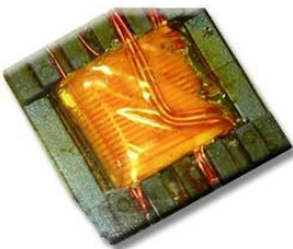
Fig. 6: Bobbin transformer with basic isolation
