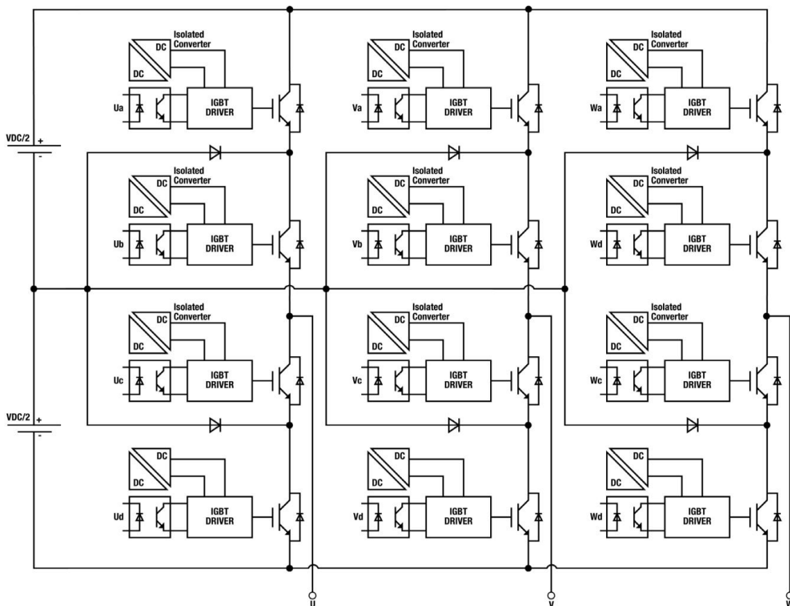
Fig. 17: 3 Phase 3-Level IGBT Inverter
