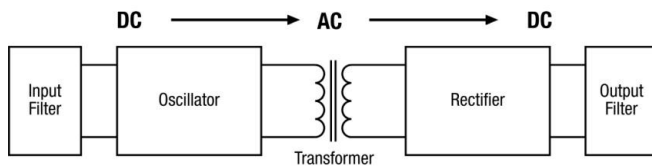
Fig. 1: Basic layout of a DC/DC-converter
