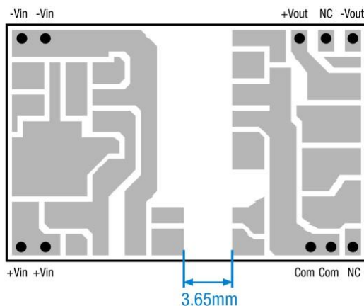
Fig. 10: Example - PCB bottom-side layout showing track separation of 3.65mm. Creepage is the minimum separation measured on both sides of the double-sided PCB.
