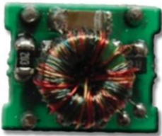
Fig. 4: Ring core transformer
