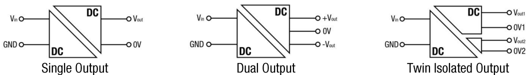
Fig. 2: Standard isolated configurations
