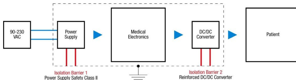
Fig. 15: Example -mains powered medical equipment requires two isolation barriers. The first is within the AC/DC power supply. The second is provided by the isolation of the DC/DC-converters.
