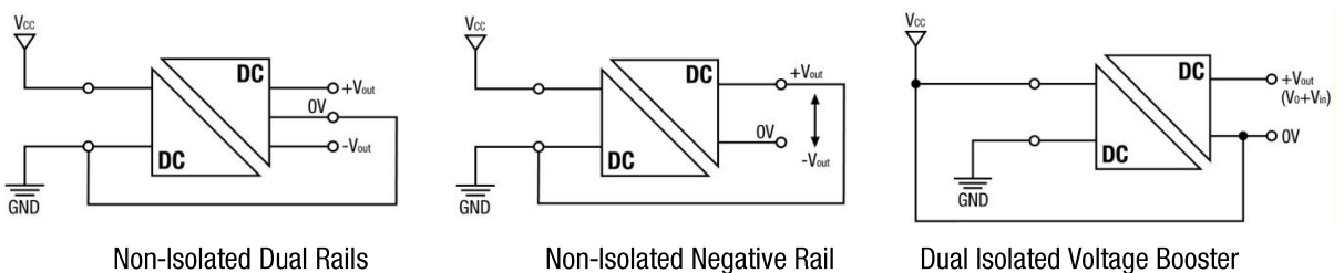
Fig. 3: Alternative supply configurations
