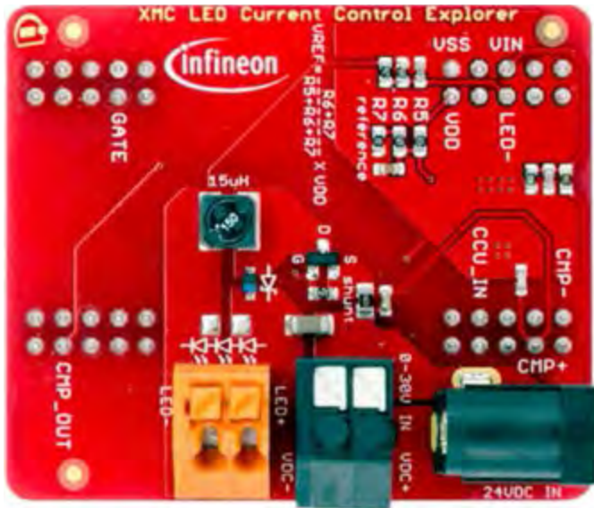
LED driver board
