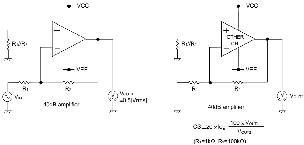
Figure 51. 測定回路 3
