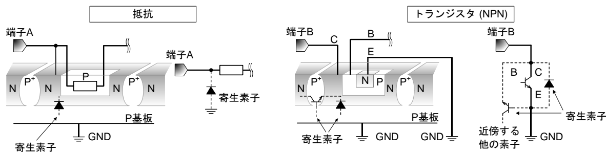
Figure 43. Example of IC Structure
